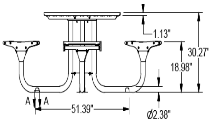
4X FOOT MOUNT
