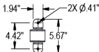
4X FOOT MOUNT
