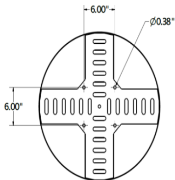
SURFACE MOUNT
