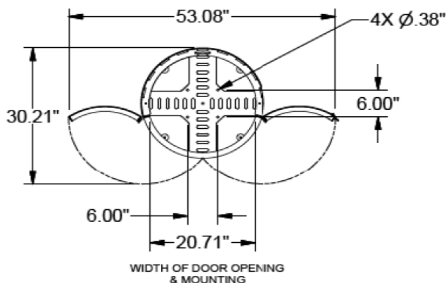
SURFACE MOUNT
