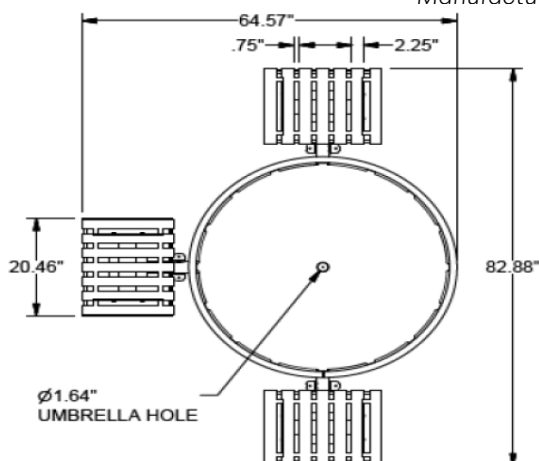
FOOT MOUNT
