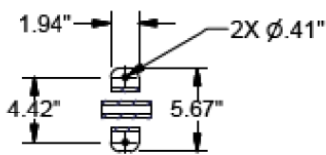
FOOT MOUNT
